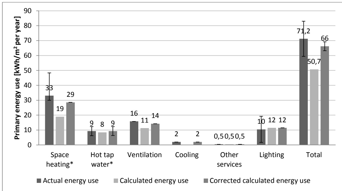
Figure 2 Actual, calculated and corrected calculated energy use in primary energy. Primary energy factor for electrical energy is 2.5. *incl. heat loss from supply systems
