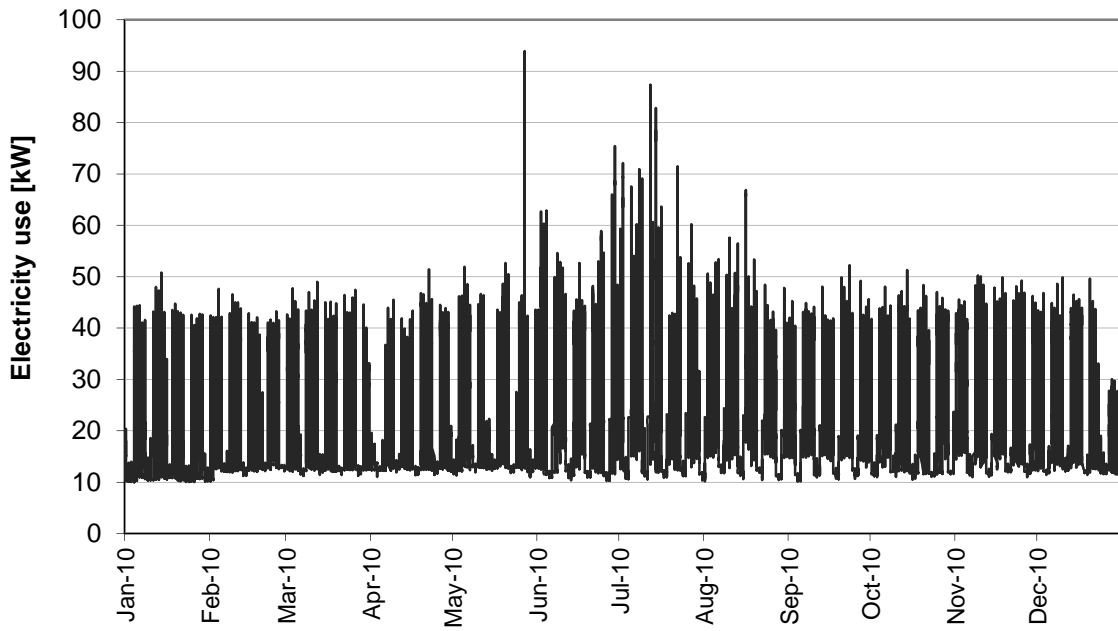
Figure 1 A plot of the total hourly electricity use for both appliances and building operation in 2010.
