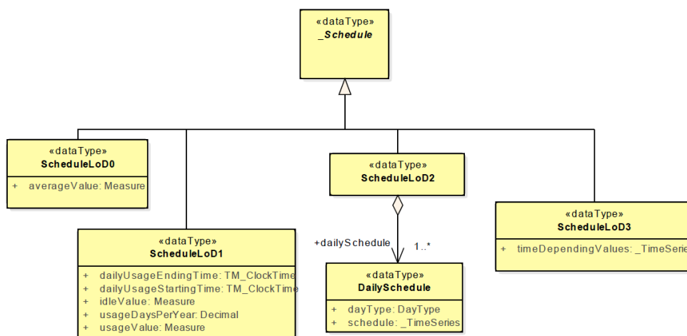
Figure 3 UML diagram extract of Schedule LoDs
