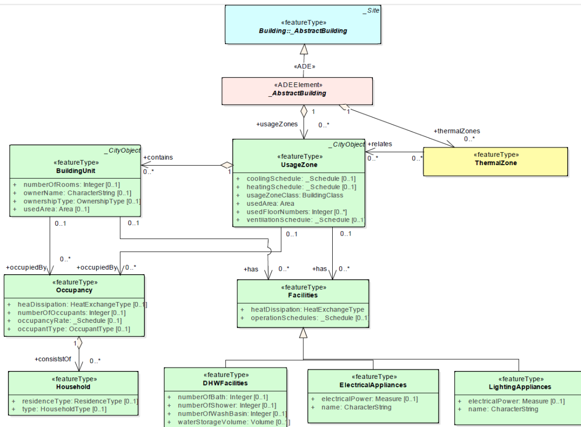
Figure 2 UML diagram extract of Occupancy Module
