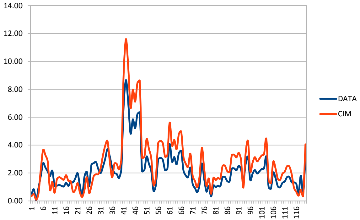
Figure 3: Time-series for the wind speed in ( m s^{-1} ) for the 5 days of simulation at 49m
