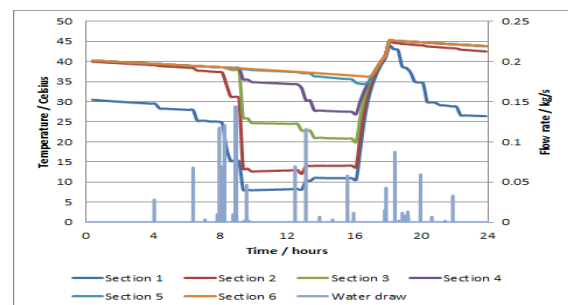
Figure 13 Tank temperatures at various heights and water draw, winter case (6 is top)
