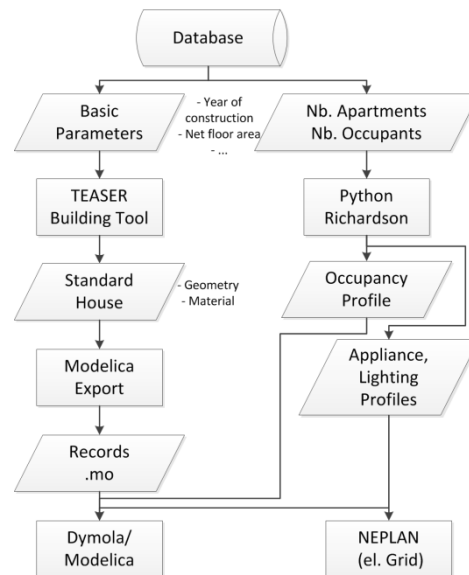
Figure 3 Modeling workflow
