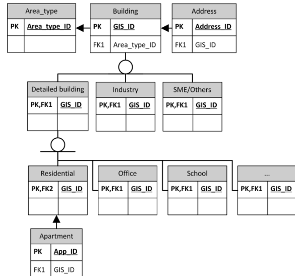
Figure 2 CIM entity relationship scheme
