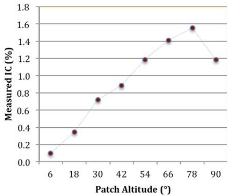
Figure 2 Mean IC values for different patch altitudes under cloudy sky conditions.
