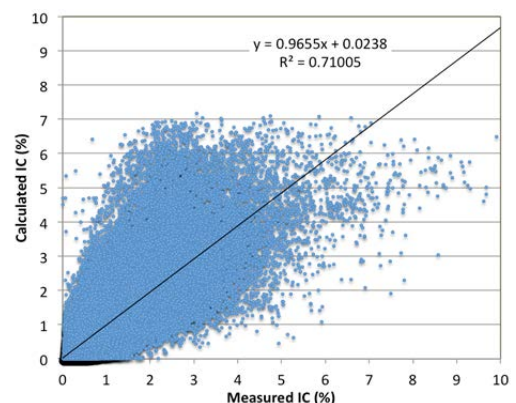
Figure 4 Measured versus calculated irradiance values for sky patches for the second data set
