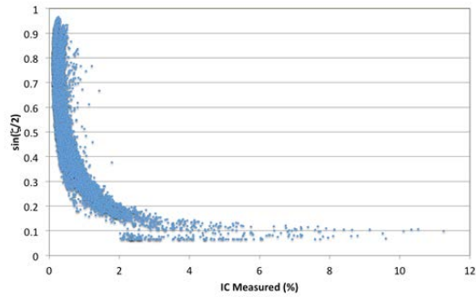
Figure 1 The relationship between measured irradiance coefficients (%) and \sin(\zeta/2) for clear sky conditions, first database.
