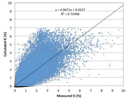
Figure 3 Measured versus calculated irradiance values for sky patches for the first data set
