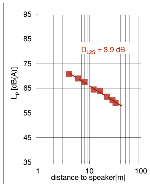
Figure 6b Measurement D_{L2,S} in existing building
