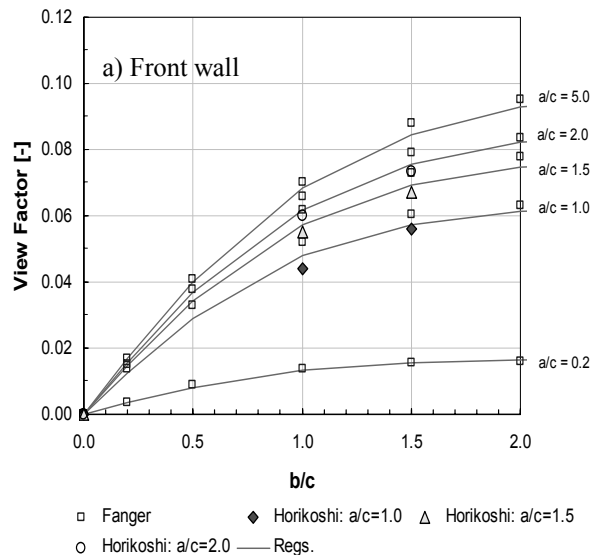
Figure 8. View factors between the whole body and planes in front of a standing person.
