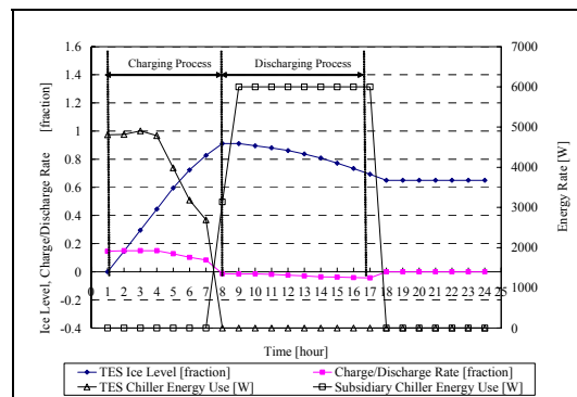
Figure 4: Performance of the TES system using chiller-priority control: charge/discharge rate, ice level and chiller energy use
