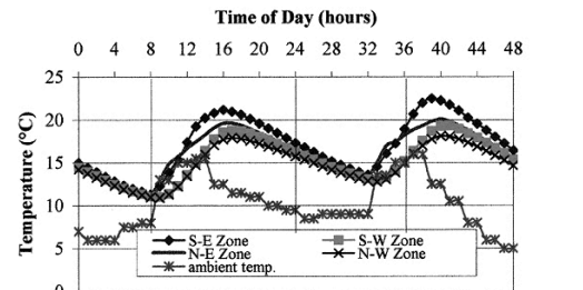
12 (a). Ambient and zone temperatures.
