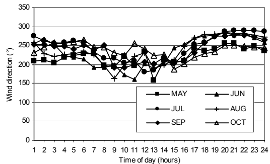
Figure 7. Mean hourly wind direction during a day for the hot months of a year. (Note: Wind direction is expressed as 0° for wind from north, 90° for east, 180° for south and 270° for west).
