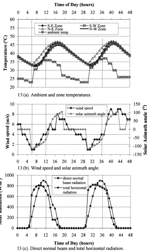
Figure 13. Zone temperatures and respective weather data, during 16 and 17 July.
