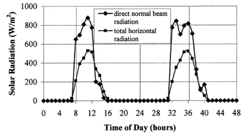
12 (c). Direct normal beam and total horizontal radiation.
