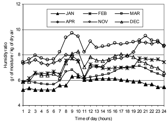
Figure 8. Mean hourly humidity ratio during a day for the cold months of a year.
