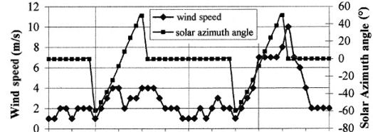
12 (b). Wind speed and solar azimuth angle.
