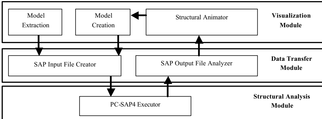
Fig. 1: VIRTUAL-SAP Software architecture
