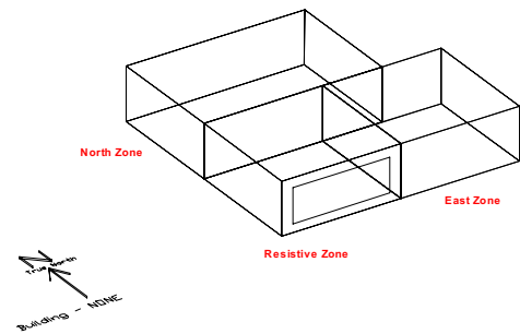
Figure 6: 3-zone building with slab-on-grade foundation.
