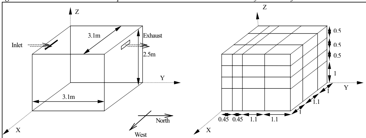
Figure 10: The MINIBAT test room partitioned into 4x3x4 = 48 cells. Three of these are jet cells.
