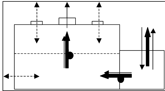
Figure 7: Air flow concept for night cooling
