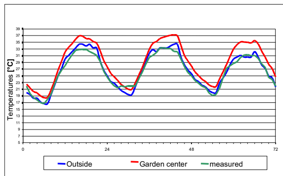
Figure 8: Temperature in garden center, measured and simulated, before optimization of input
