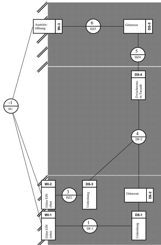
Figure 12: Network model of the air flow calculation
