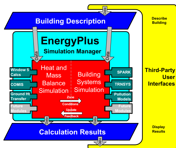
Figure 1. Overall EnergyPlus Structure
