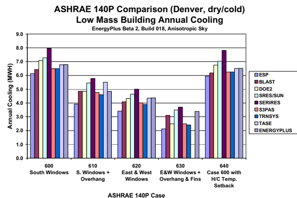
Figure 2. Sample EnergyPlus Comparative Testing Results
