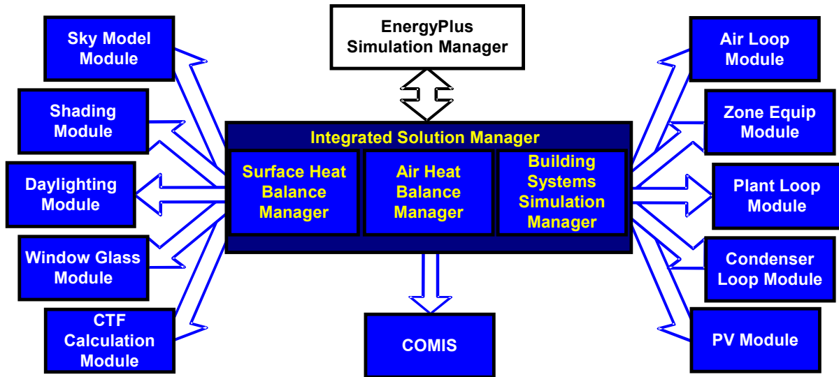
Figure 2. Integrated EnergyPlus Solution Manager Featuring the Heat Balance Modules.
