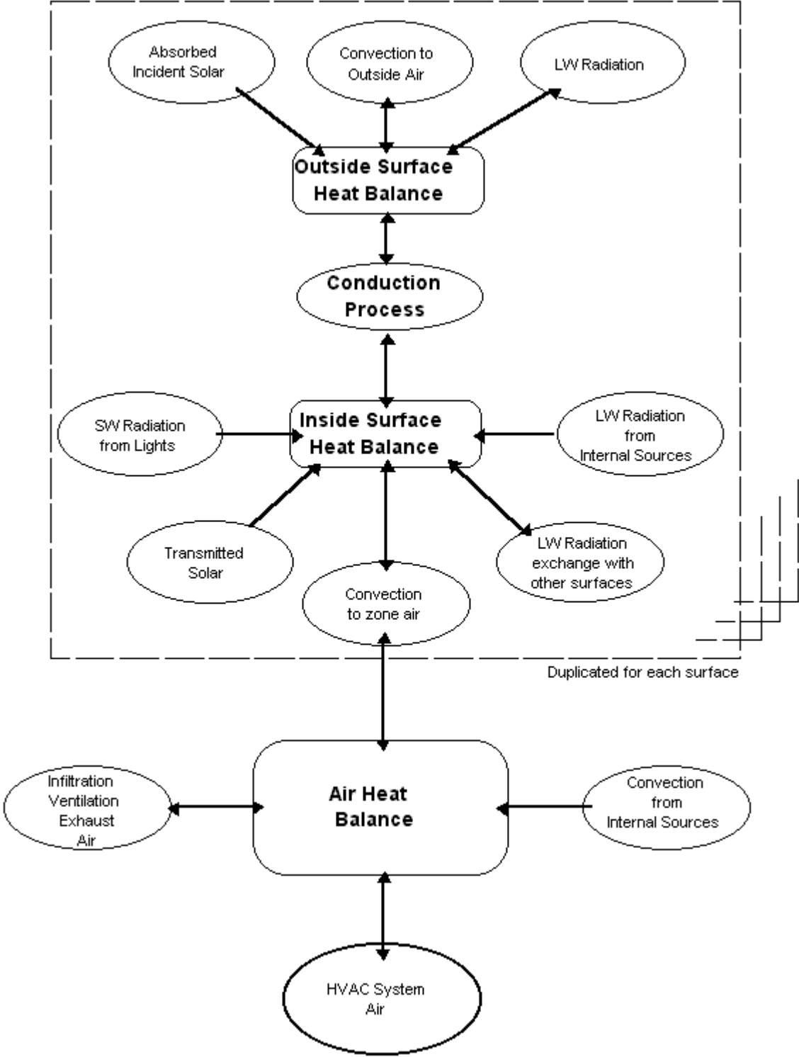
Figure 1. Schematic of the Energy Balance Processes in a Zone (Pedersen 1997).
