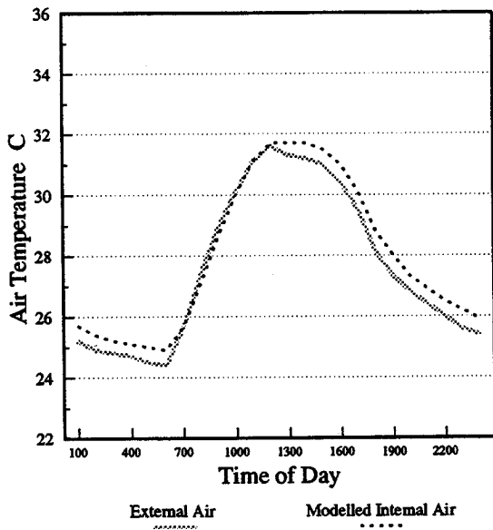
Figure 10 Modelled Air Temperatures for Average Day, Proposed Low Cost House, Ground Floor.
