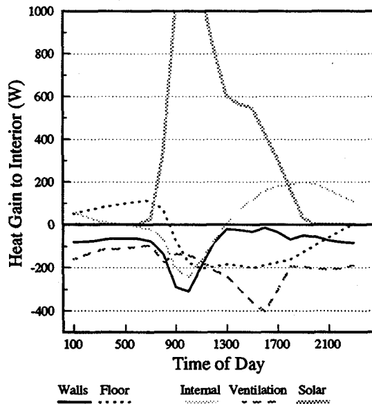
Figure 8 Modelled Energy Flows for Average Day, Modern Cluster-Link House, Ground Floor.
