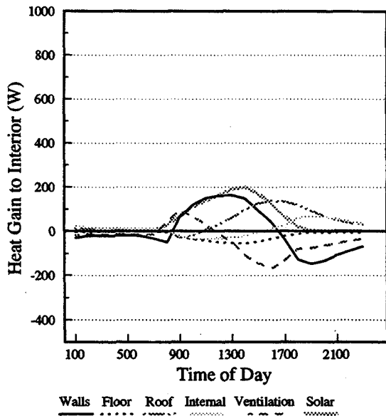
Figure 7 Modelled Energy Flows for Average Day, Traditional Attap Roof House, Main Living Space.
