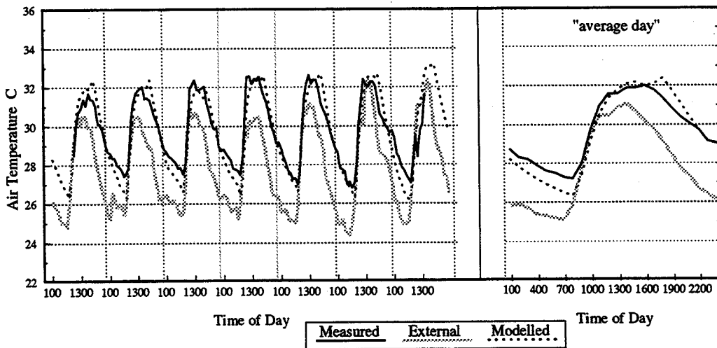
Figure 5 Comparison of Measured and Modelled Air Temperatures in Main Living Space; Modern Cluster-Link House
