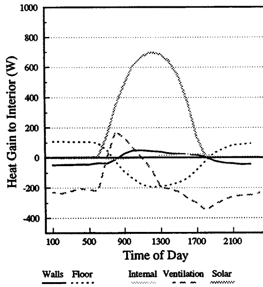
Figure 11 Modelled Energy Flows for Average Day, Proposed Low Cost House, Ground Floor.
