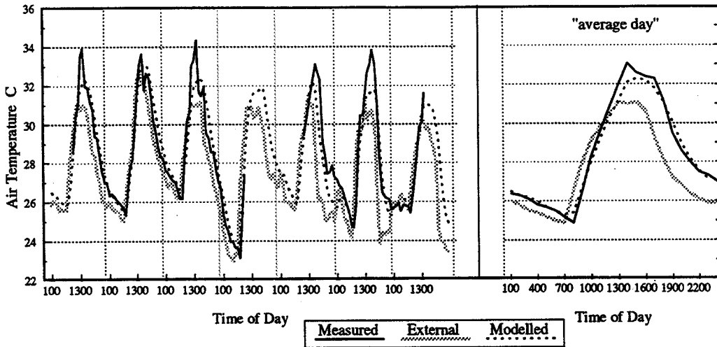
Figure 4 Comparison of Measured and Modelled Air Temperatures in Main Living Space; Traditional Attap Roof House
