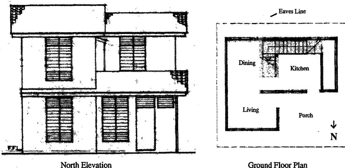
Figure 9 Proposed Low Cost Housing Design (Universiti Sians Malaysia 1992)
