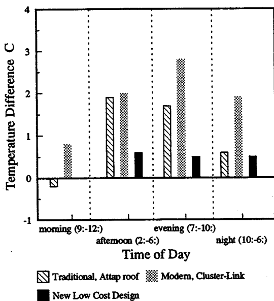
Figure 6 Modelled Period Average Inside to Outside Temperature Differences
