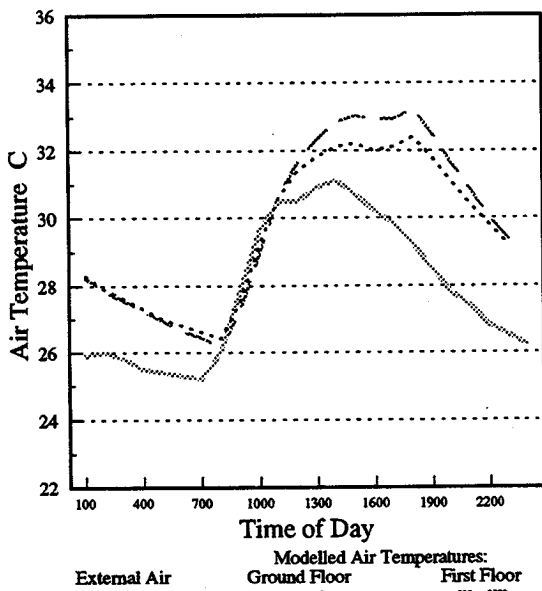
Figure 12 Modelled Air Temperatures for Average Day, Cluster-Link House, Showing Upstairs Rooms.
