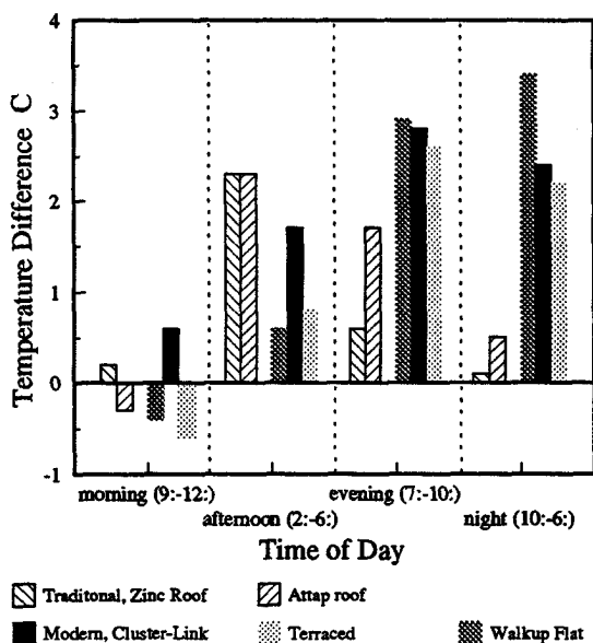
Figure 3 Period Average Inside to Outside Temperature Differences for the Measured Cases.
