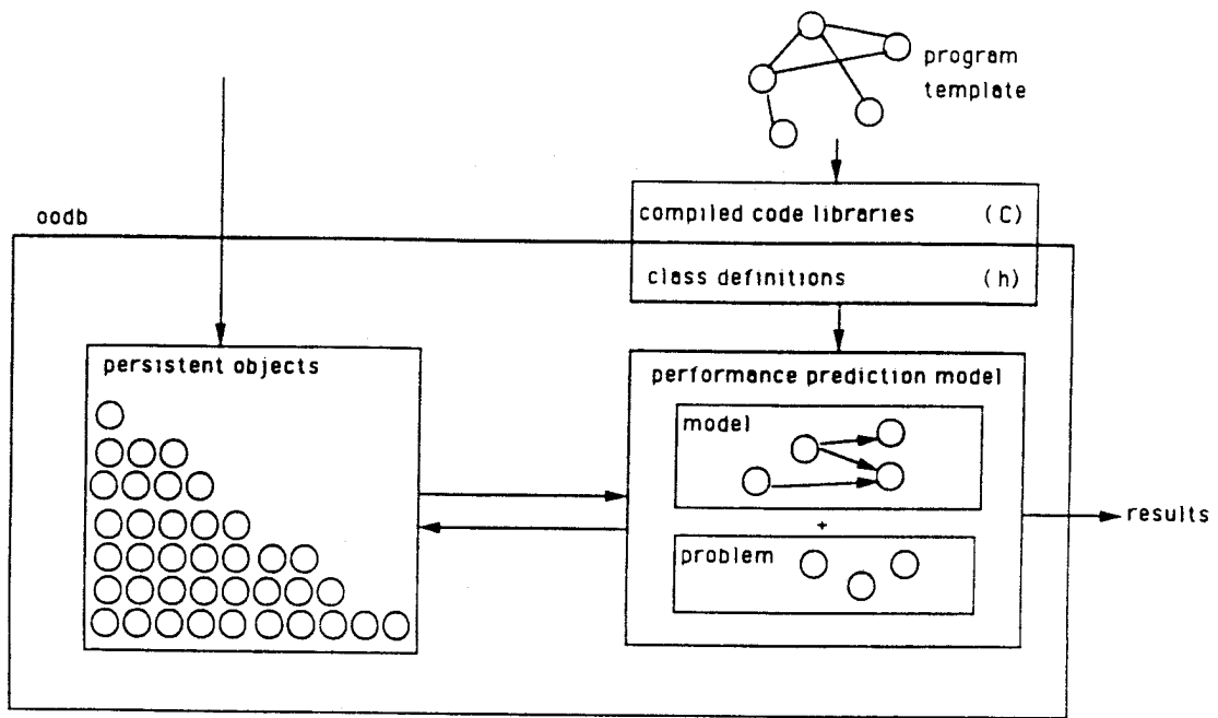
Fig. 1. System Architecture of the EKS.
