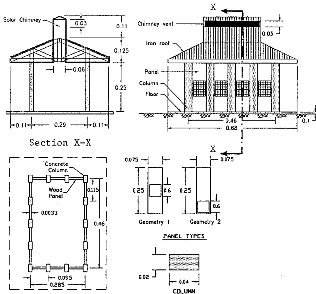
Figure 1. Details and dimensions (m) of the 1/12th scale model.
