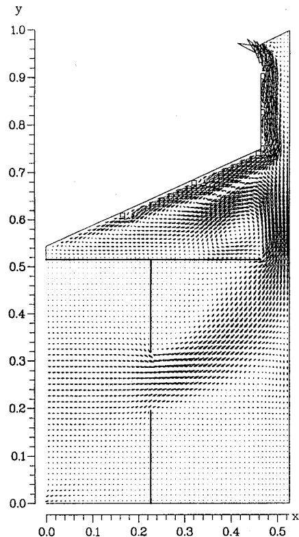
Figure 4. Computational velocity streaklines.
