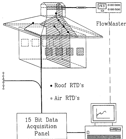
Figure 3. Data acquisition system and location of temperature sensors. Dashed area denotes 2-D computational domain.
