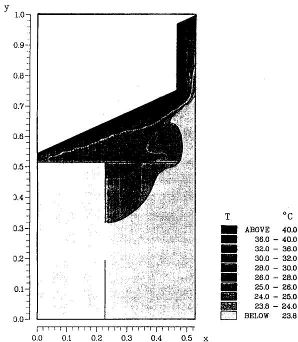
Figure 6. Map of the computed temperature field.
