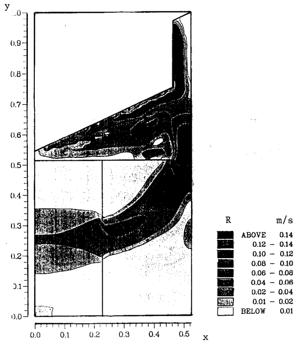
Figure 5. Shadowgraph representation of velocity field. [R = (V^2 + U^2)^{1/2}]
