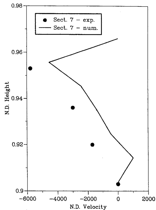
Figure 7. Predictions and experimental data for the velocities at the outlet section (Section #7).
