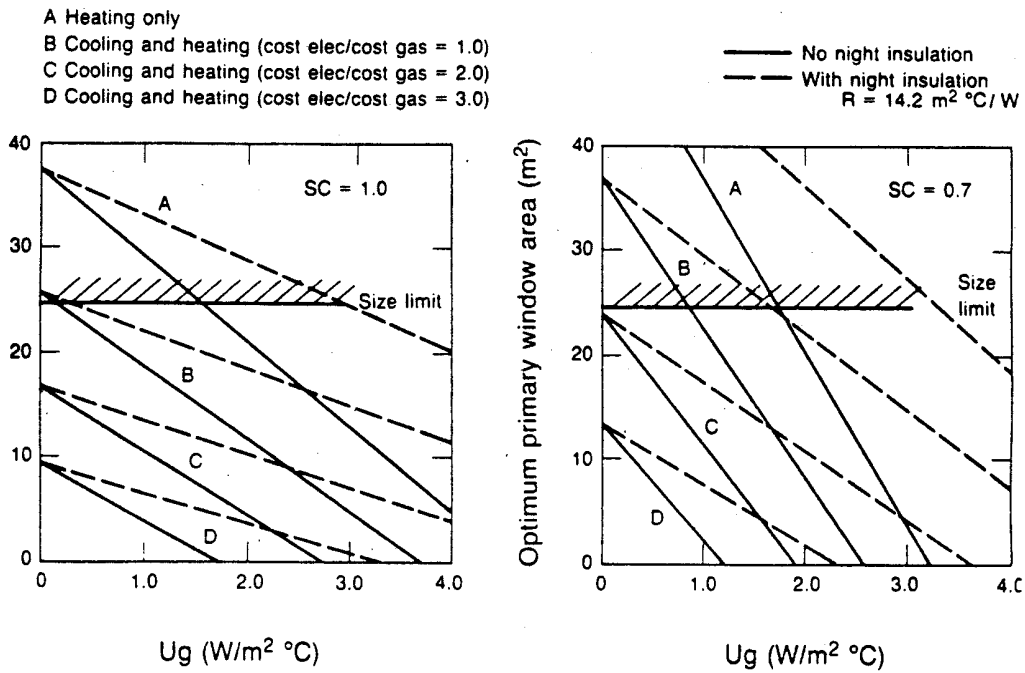
Fig. 3. Primary window size as a function of U-value, night insulation, and ratio of the cost of electricity (cooling) to the cost of gas (heating) for two shading coefficients for a south orientation in Madison, Wisc.
