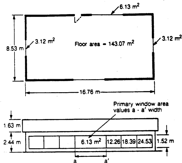
Fig. 1. Residential model description.
