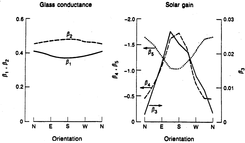
Fig. 2. Residential heating energy regression coefficients for Madison, Wisc., as a function of primary window orientation.
