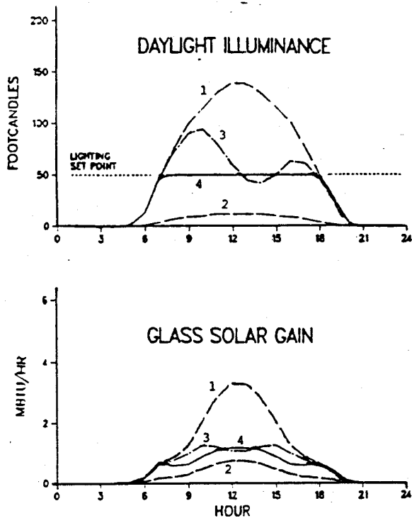
Fig. 13. DOE-2 calculation of daylight illuminance and solar gain in a south-facing sidelit office module for a clear day in Madison, WI. Four different glass types are compared -- (1) conventional, high-transmittance clear glass ( VT=78\% ); (2) conventional, low-transmittance reflective glass ( VT=7\% ); (3) hypothetical photochromic glass whose transmittance decreases from 78% to 20% as incident solar radiation increases; and (4) hypothetical electrochromic glass whose transmittance is modulated hour by hour to just meet a 50 fc illuminance setpoint.
