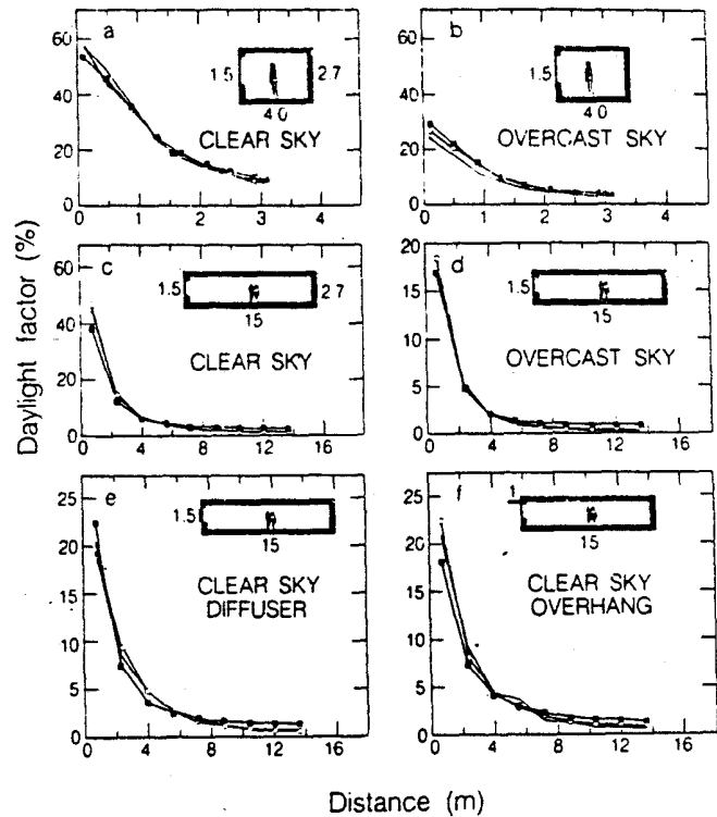
Fig. 9. (a)-(f): SUPERLITE (O) and DOE-2 (□) predictions for interior/exterior illuminance ratio compared with sky-simulator measurements (-) made along centerline of different scale models. Cases of clear sky have solar altitude 50^\circ , azimuth 0^\circ , but exclude direct sun. Ground reflectance is zero. Interior reflectances are 25% for floor, 60% for walls, 80% for ceiling. Glass transmittance is 90%; diffuser transmittance in (e) is 60%.
