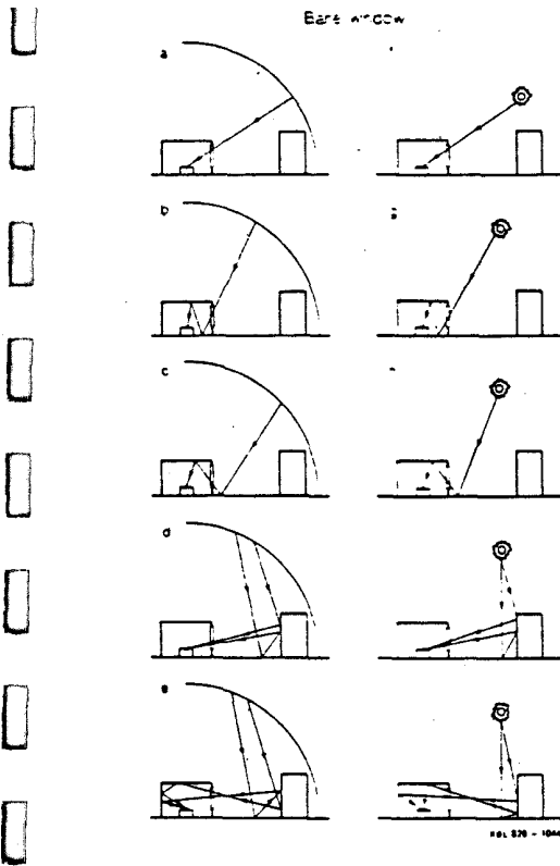
Fig. 1. Paths by which light originating from sky (a-e) and from sun (f-j) can reach workplane through a transparent window without a shading device.
