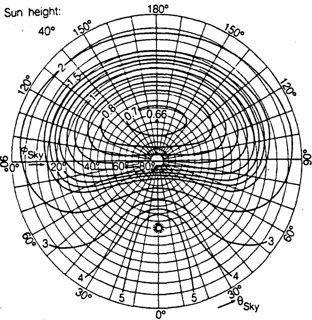
Fig. 3. Clear sky luminance distribution (normalized to unit zenith luminance) for a solar altitude of 40°.
