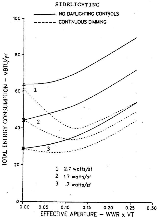
Fig. 10. DOE-2 prediction of total annual energy consumption vs. effective aperture (window-to-wall ratio times visible transmittance) for a south-facing sidelit office module in Los Angeles, with and without daylighting controls for different lighting power densities.
